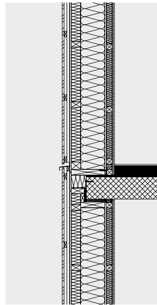
Beton/HSB_Stütze in Aussenwand
